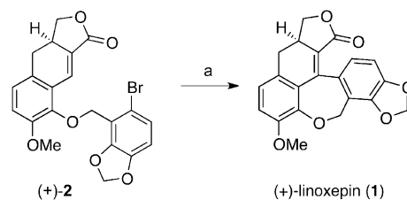
Scheme 8. Synthesis of (+)-linoxepin ( 1 ). a) \text{PdCl}_2 (20 mol%), \text{PPh}_3 (44 mol%), \text{CsOAc} (10.0 equiv), DMF, 75^\circ\text{C} , 4 h, 76%.
