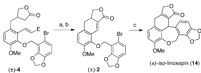
Scheme 6. Undesired formation of (±)-iso-linoxepin ( 14 ). a) \text{OsO}_4 , \text{NaIO}_4 , TEBAc, \text{THF}/\text{H}_2\text{O} 5:3, RT, 98%; b) \text{TiCl}_4 , \text{NEt}_3 , \text{CH}_2\text{Cl}_2 , -78^\circ\text{C} \rightarrow -25^\circ\text{C} \rightarrow \text{RT} , 3 h, 49%; c) \text{PdCl}_2 (20 mol%), \text{PPh}_3 (44 mol%), \text{NEt}_3 (10 equiv), microwave radiation, DMF, 130^\circ\text{C} , 7 h, 74%; \text{E} = \text{CO}_2t\text{Bu} , TEBAc = triethylbenzylammonium chloride.
