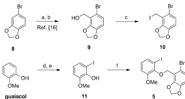
Scheme 3. Synthesis of the aryl iodide 5 . a) i) HNiPr 2 , n BuLi, THF, –78 °C, 1 h; ii) DMF, THF, –78 °C → RT, 95%; b) NaBH 4 , THF, reflux, 90 min, 97%; c) TMSCl, NaI, CH 3 CN, RT, 1 h, 99%; d) DHP, PPTS, CH 2 Cl 2 , RT, 4 h, 95%; e) i) n BuLi, THF, RT, 7 h; ii) I 2 , THF, –50 °C → RT, 16 h, 98%; f) 10 , K 2 CO 3 , acetone, reflux, 94%. DHP = 3,4-dihydro-2 H -pyran; PPTS = pyridinium p -toluenesulfonate.
