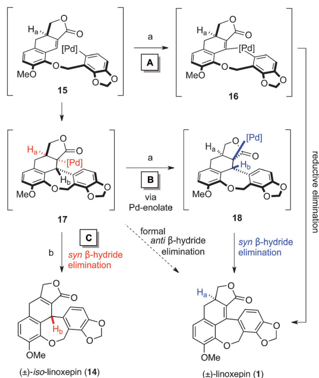
Scheme 7. Mechanistic rationale for the formation of (±)- 1 and (±)- 14 . [21] 15 was obtained by the oxidative addition of \text{Pd}^0 to (±)- 2 ; pathway A : C–H activation pathway by highly electrophilic Ar–Pd species; pathway B : Generation of a syn \beta -hydride ( \text{H}_b ) by a Pd-enolate; Pathway C : Formation of (±)-iso-linoxepin 14 by a syn \beta -hydride elimination of \text{H}_a ; conditions: a) \text{PdCl}_2 (20 mol%), \text{PPh}_3 (44 mol%), \text{NEt}_3 (10 equiv), microwave radiation, DMF, 130^\circ\text{C} , 7 h, 74%; b) \text{PdCl}_2 (20 mol%), \text{PPh}_3 (44 mol%), \text{CsOAc} (10.0 equiv), DMF, 75^\circ\text{C} , 4 h, 78%.
